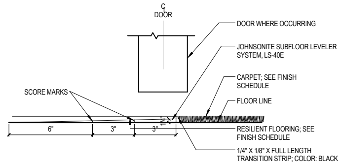
D. FLOORING TRANSITION - RESILIENT / CARPET
