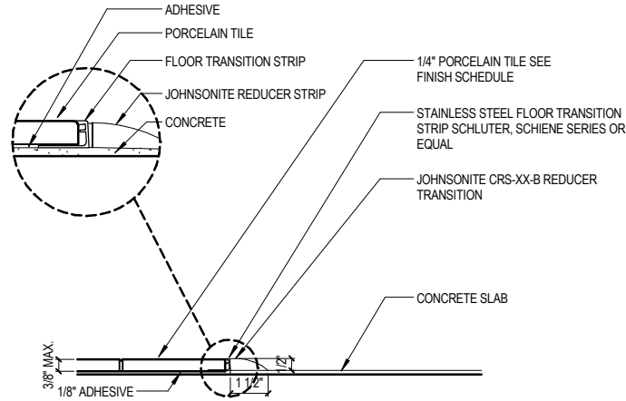
C. FLOORING TRANSITION - PORCELAIN TILE / CONCRETE FLOORING NO THRESHOLD
