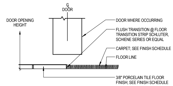
E. FLOORING TRANSITION - PORCELAIN TILE / CARPET NO THRESHOLD
