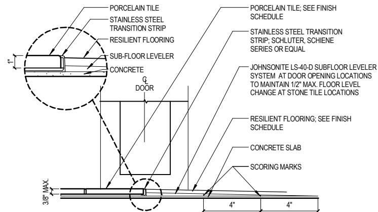
A. FLOORING TRANSITION - PORCELAIN TILE / RESILIENT FLOORING NO THRESHOLD
