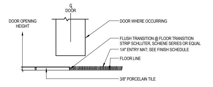
G. FLOORING TRANSITION - ENTRY MAT / PORCELAIN TILE NO THRESHOLD
