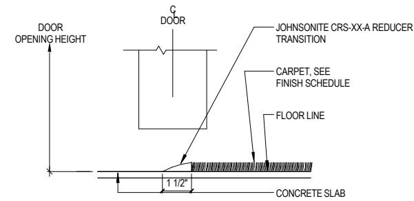
F. FLOORING TRANSITION - CONCRETE / CARPET NO THRESHOLD
