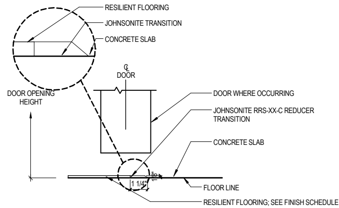
B. FLOORING TRANSITION - RESILIENT / CONCRETE FLOORING
